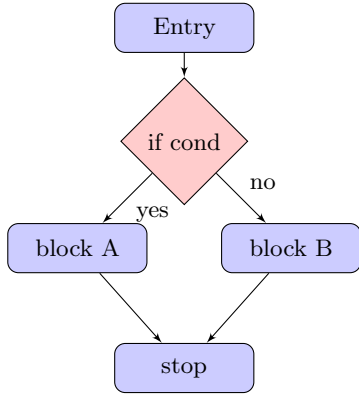
Figure 8: Example of a diamond formula
